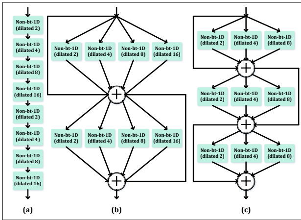
Fig. 4. Sequential and hierarchical architectures of dilated Non-bottleneck-1D (Non-bt-1D) layers. From left to right: (a) Sequential architecture, (b) 4 \times 2 hierarchical architecture, (c) 3 \times 3 hierarchical architecture.
