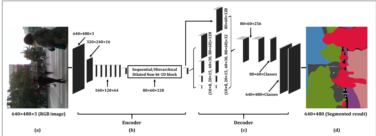
Fig. 3. The proposed architecture. (a) Input, (b) Encoder, (c) Decoder, (d) Prediction.
